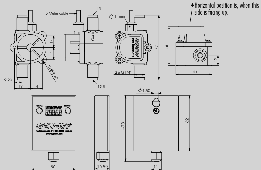
Battery-change: battery-type: CR 2032
